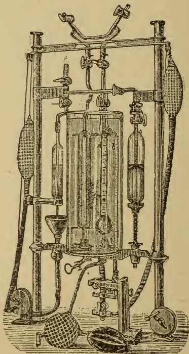
Fig. 96. APPARATUS FOR QUICK ANALYSIS OF AIR, ETC.
